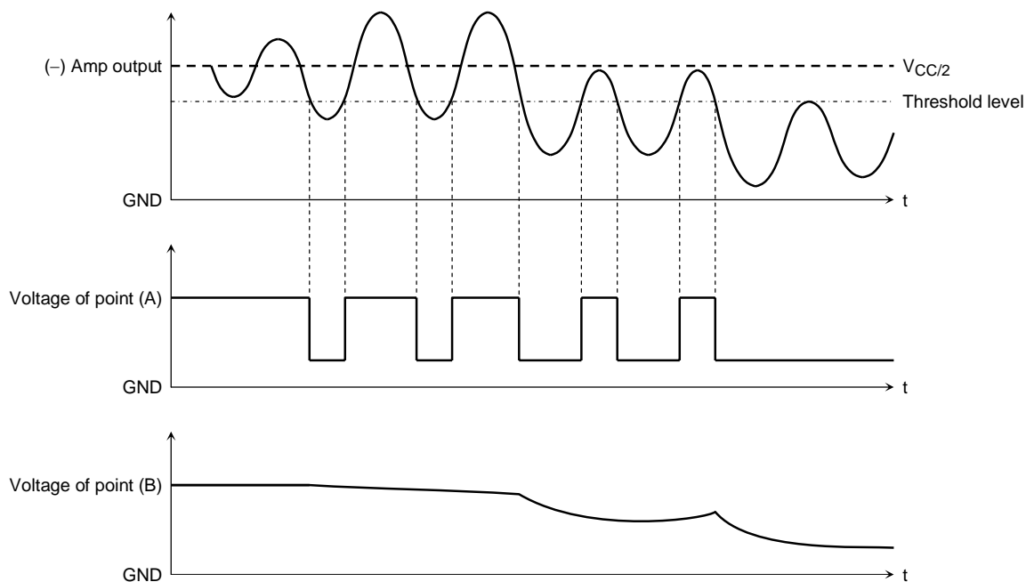
Figure 10 Wave Form
