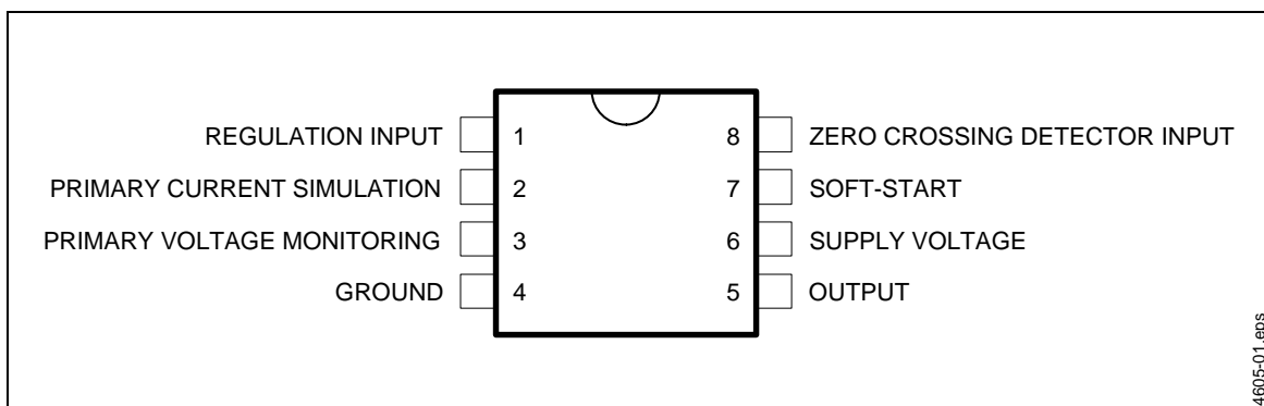
Figure 1. Pin Connections
