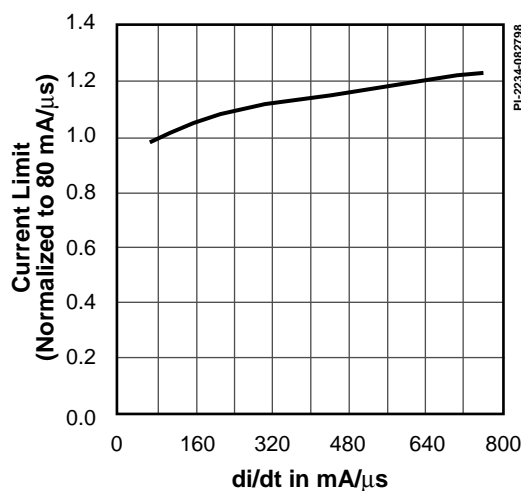
TNY255 CURRENT LIMIT vs. di/dt
