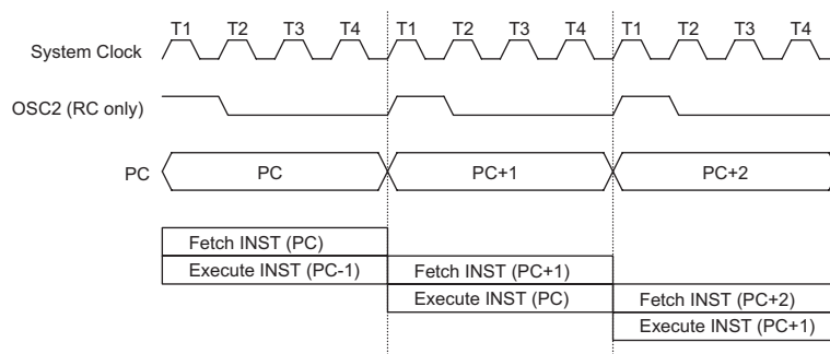
Execution Flow
