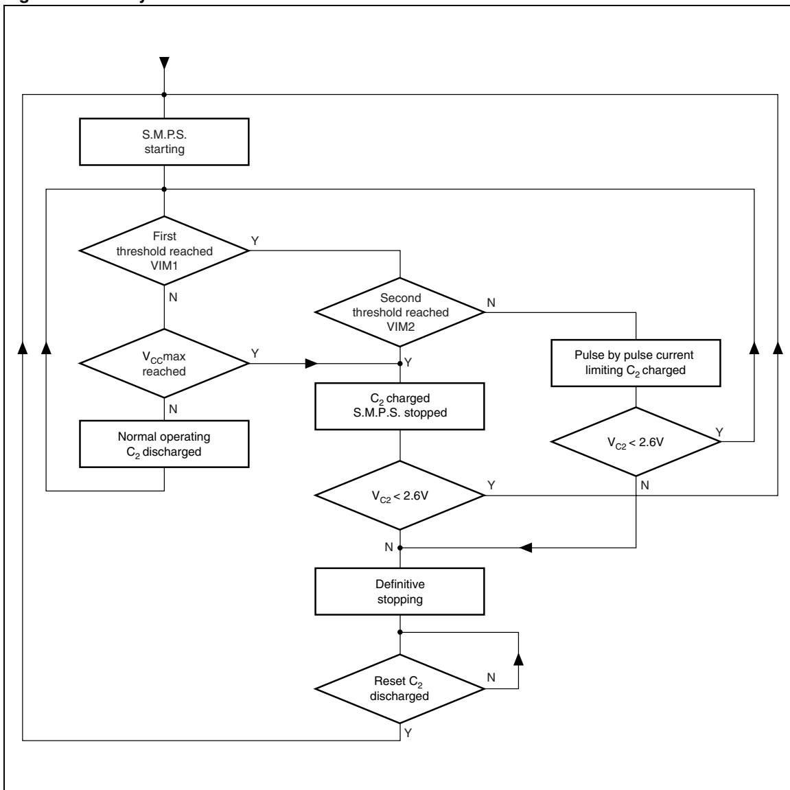
Figure 7. Security Flow-chart
