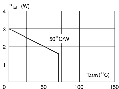
Figure 4. Maximum Power Dissipation
