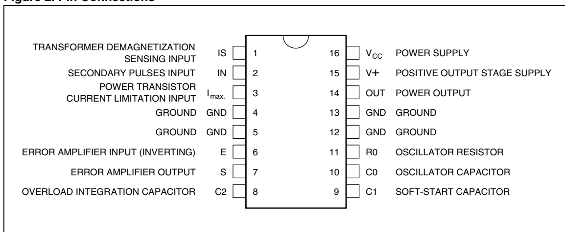
Figure 2. Pin Connections
