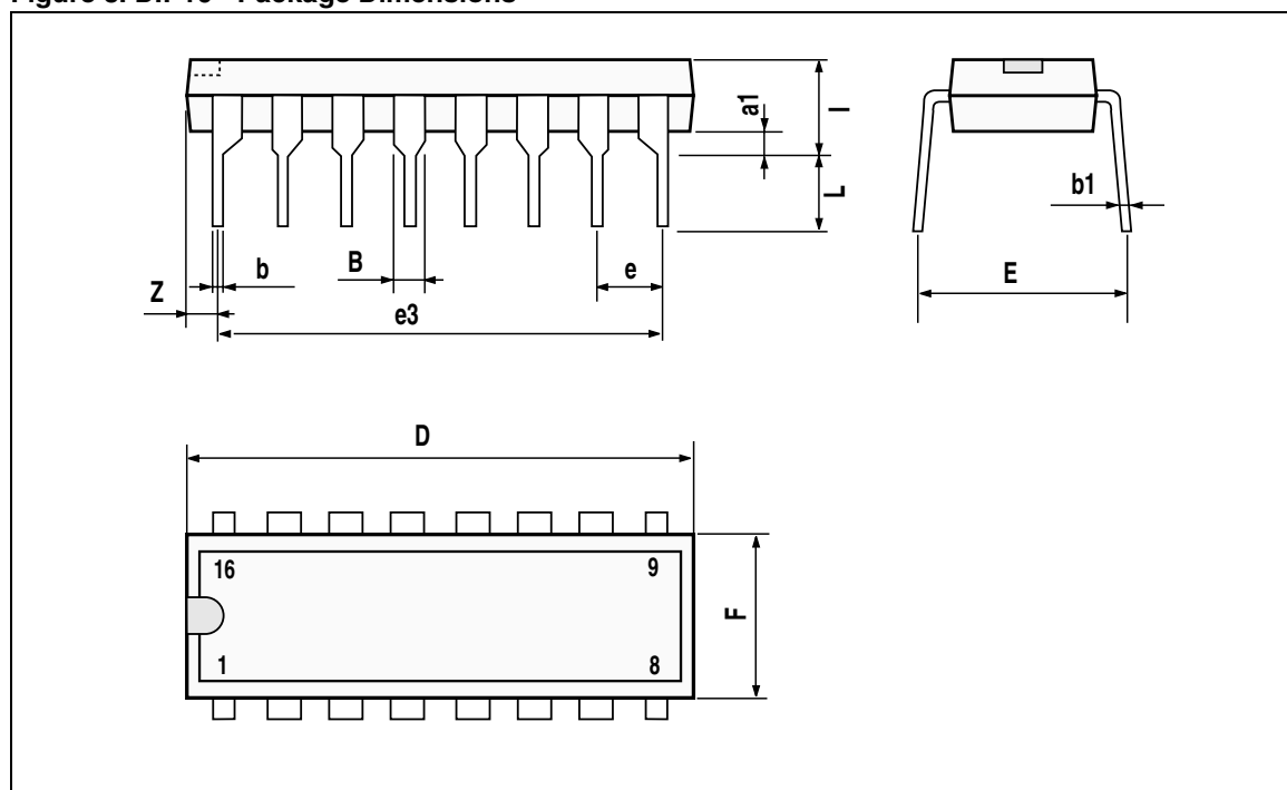
Figure 8. DIP16 - Package Dimensions
